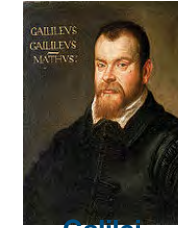
Galilei Galilei ~1500
