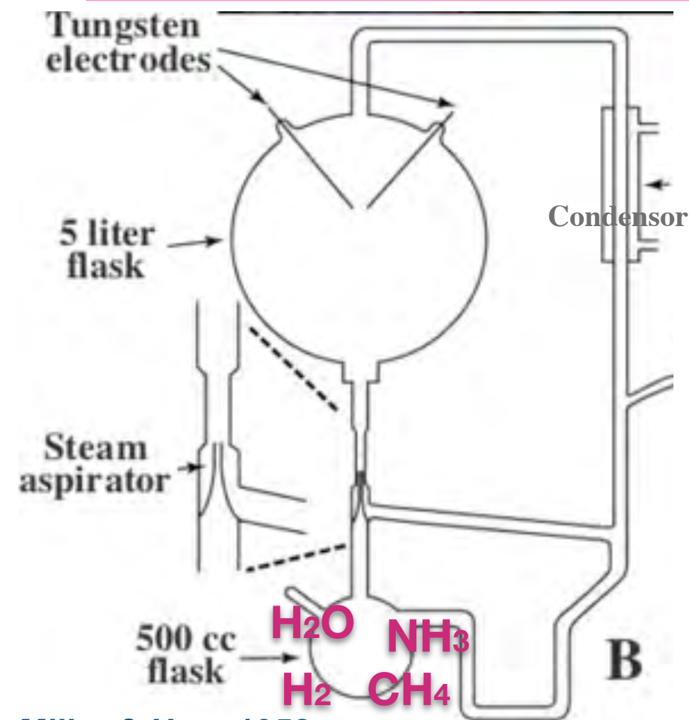
Stanley Miller 1952
