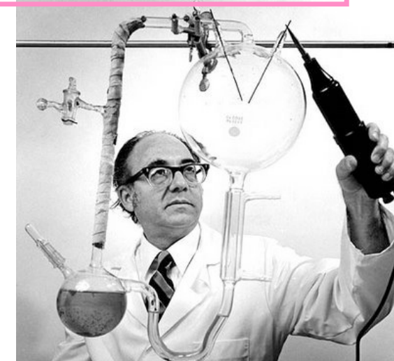
Stanley Miller 1952
